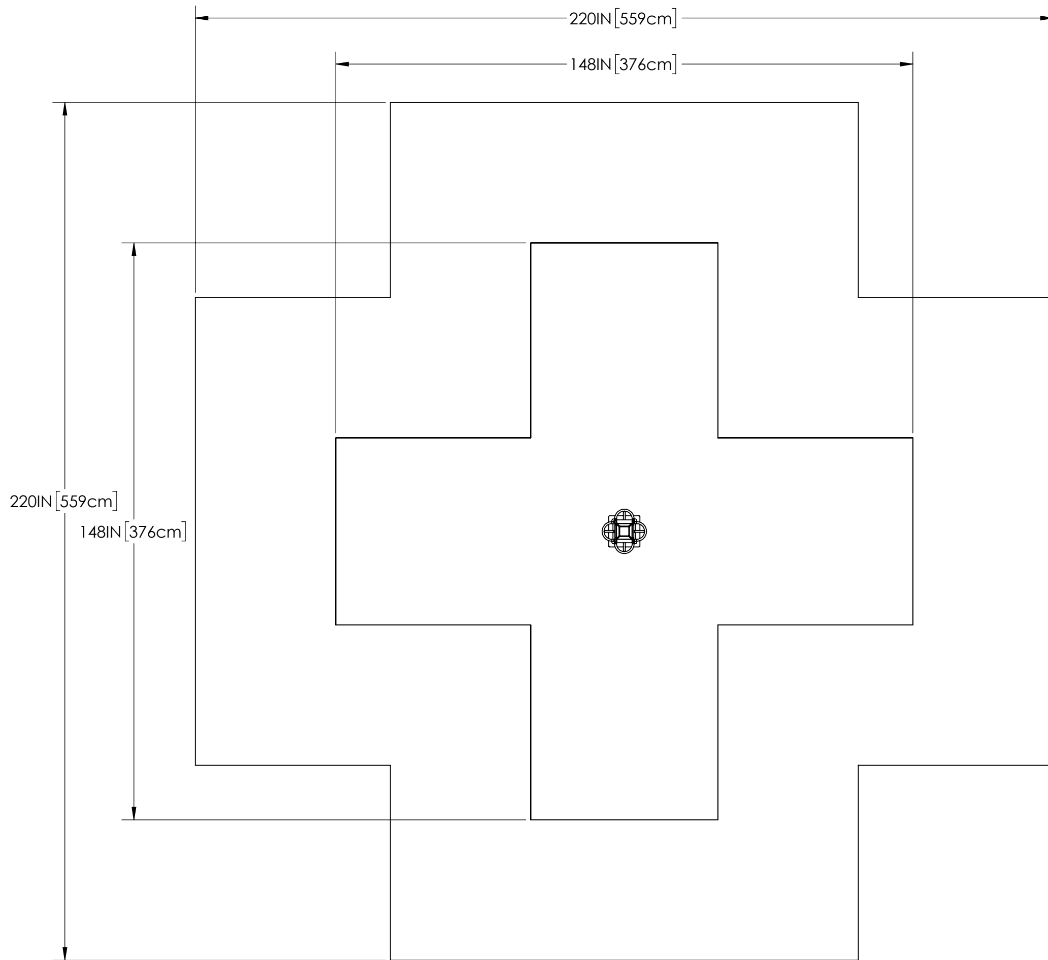
PLAN VIEW
