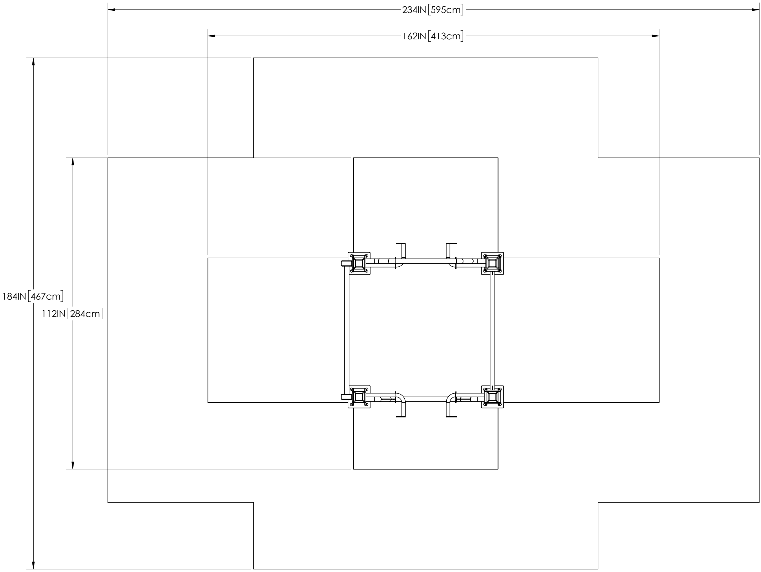
PLAN VIEW
