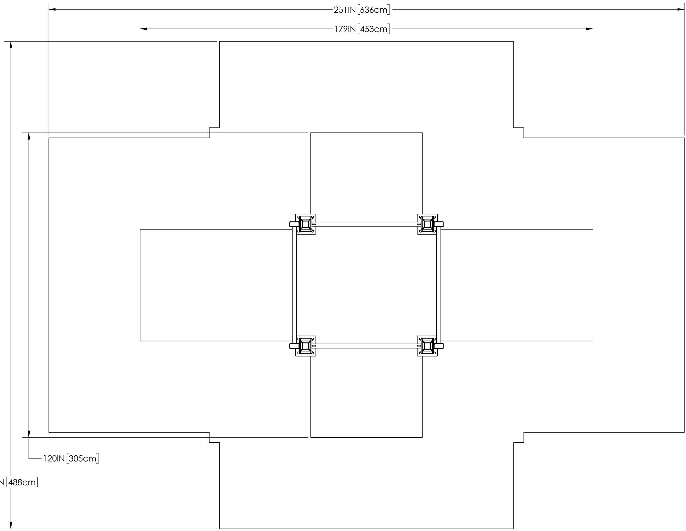
PLAN VIEW
