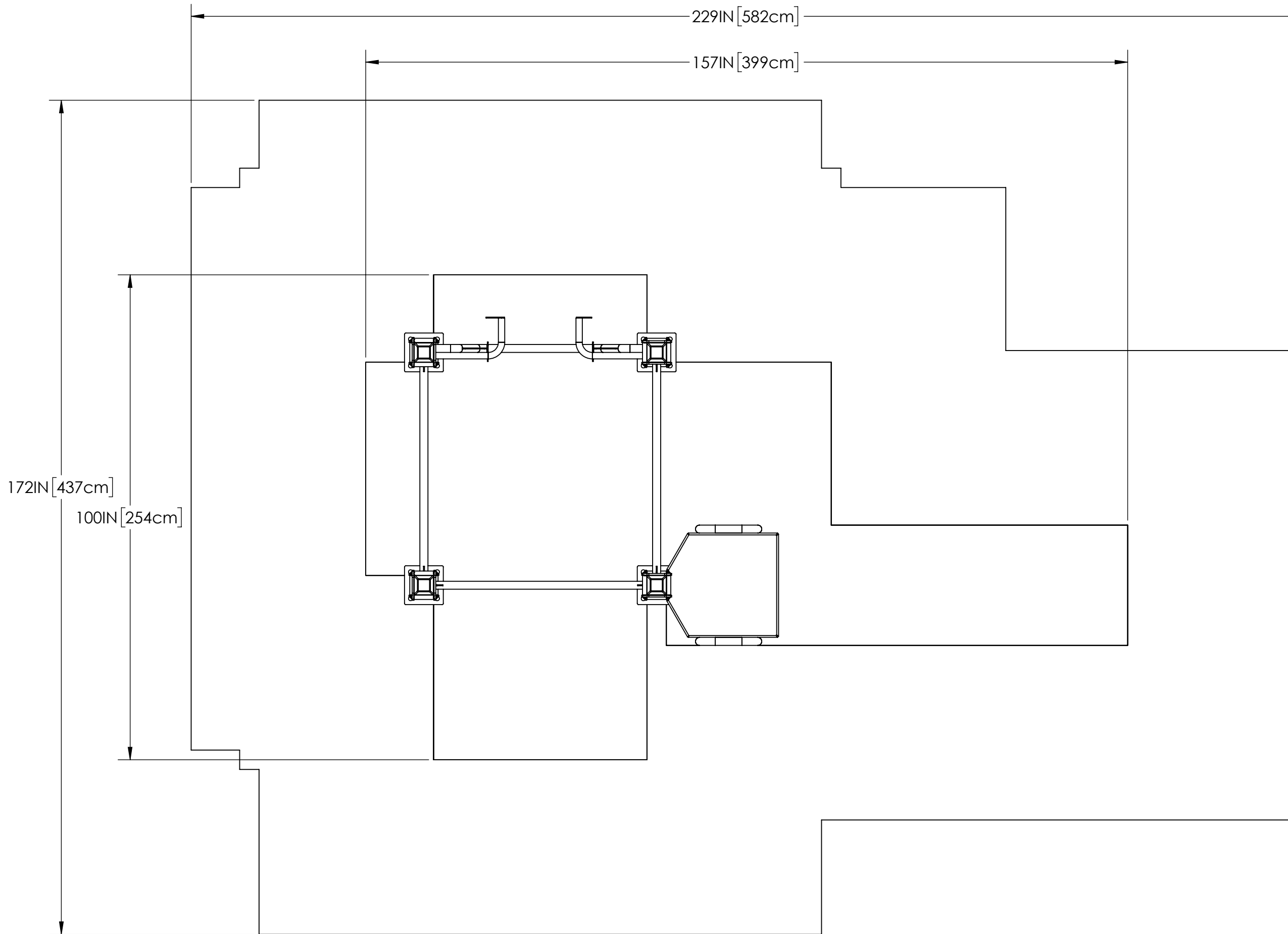
PLAN VIEW
