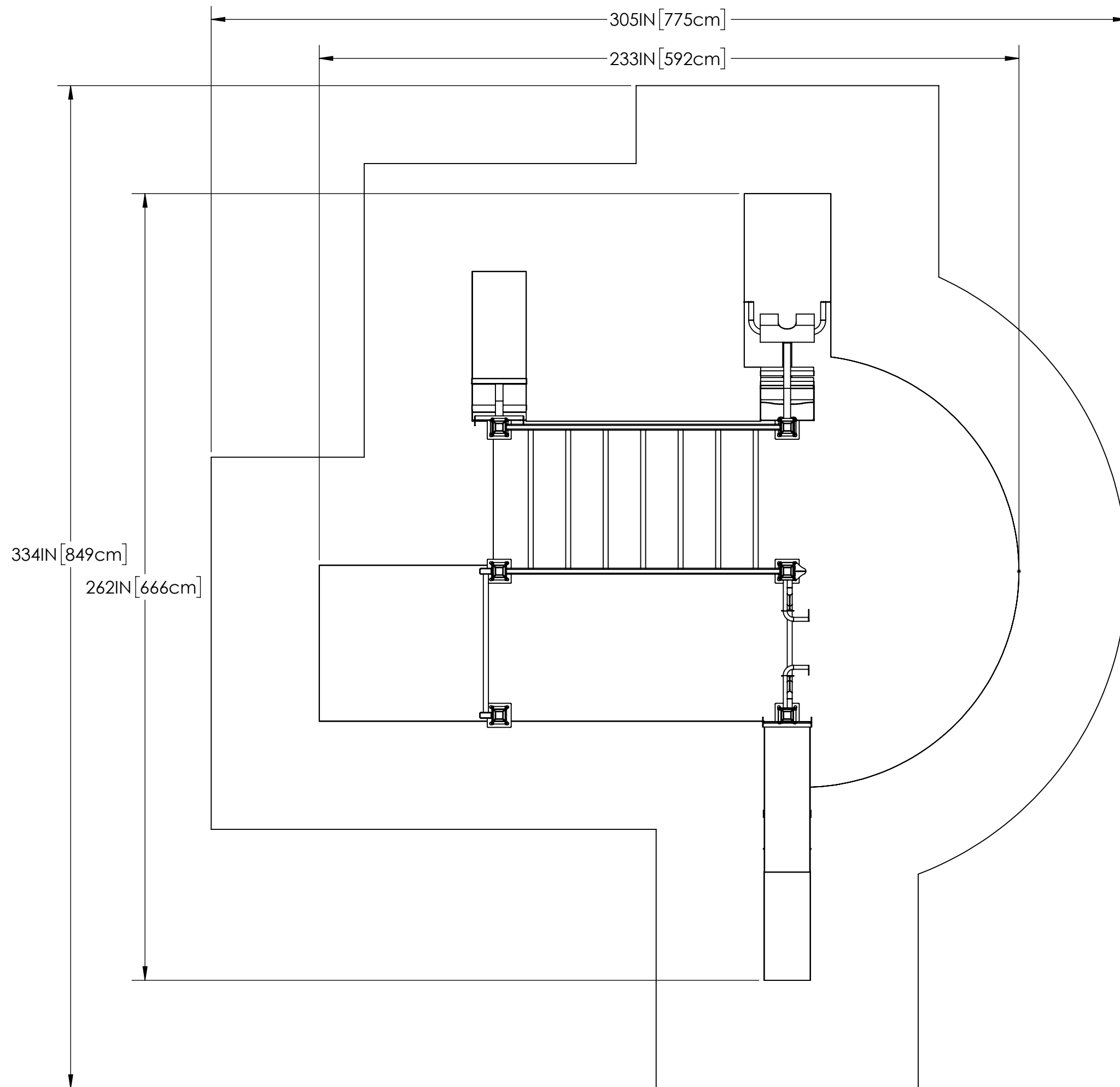
PLAN VIEW
